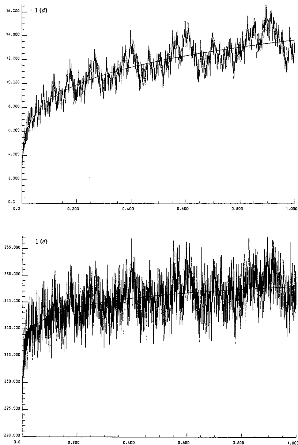
FIGURE 1. Weierstrass–Mandelbrot cosine fractal function C(t) , range 0 \leq t \leq 1 , \gamma = 1.5 : (a) D = 1 ; (b) D = 1.2 ; (c) D = 1.5 ; (d) D = 1.8 ; (e) D = 1.99 (note change of origin).
