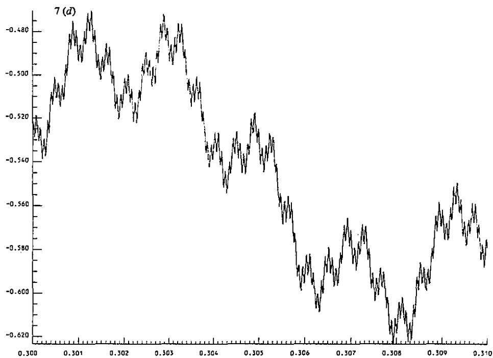
FIGURE 7. Weierstrass-Mandelbrot fractal function, range 0.30 \leq t \leq 0.31 , D = 1.5 : (a) A(t) , \gamma = 1.2 ; (b) A(t) , \gamma = 5 ; (c) random, \gamma = 1.2 ; (d) random, \gamma = 5 .
