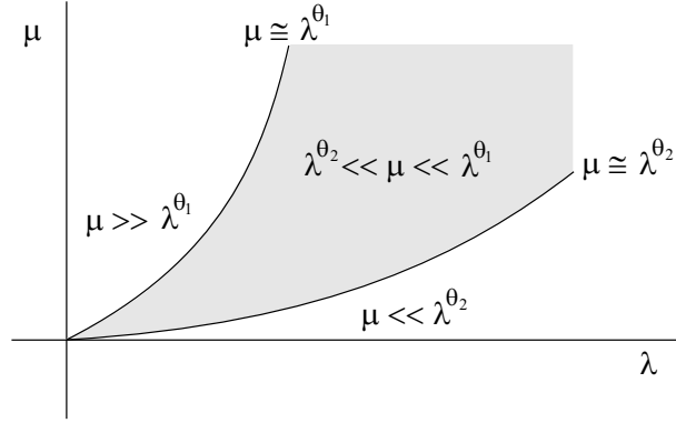
FIGURE 1. A symbolic drawing of the five regions describing the change in the regime for the asymptotic behavior of the solutions (u_{\lambda,\mu}, v_{\lambda,\mu}) as (\lambda, \mu) \rightarrow (0,0) . The shadowed area in the middle stands for the region for solutions that bifurcate from u = 0, v = 0 .
