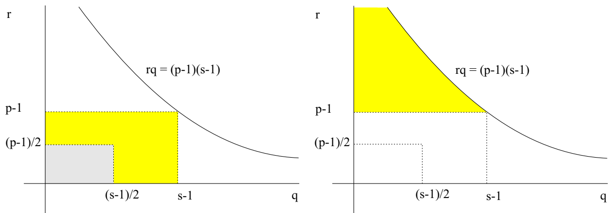
FIGURE 3. On the left we highlight the regions of parameters corresponding to the asymptotic behaviors described in points i) and ii) of Theorem 5 and on the right the parametric regime leading to the behavior in iii).
