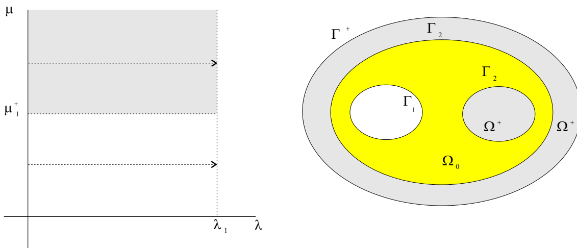
FIGURE 2. A possible configuration for \Omega : \Omega^+ has two components, the outer one with \mu_1^+ < \infty , the inner one with \mu_2^+ = \infty , while \lambda_1 < \infty . For \mu \leq \mu_1^+ the solution (u_{\lambda,\mu}, v_{\lambda,\mu}) \rightarrow (\infty, 0) as \lambda \rightarrow \lambda_1 while it keeps a finite profile in the outer component as \lambda \rightarrow \lambda_1 provided \mu > \mu_1^+ .
