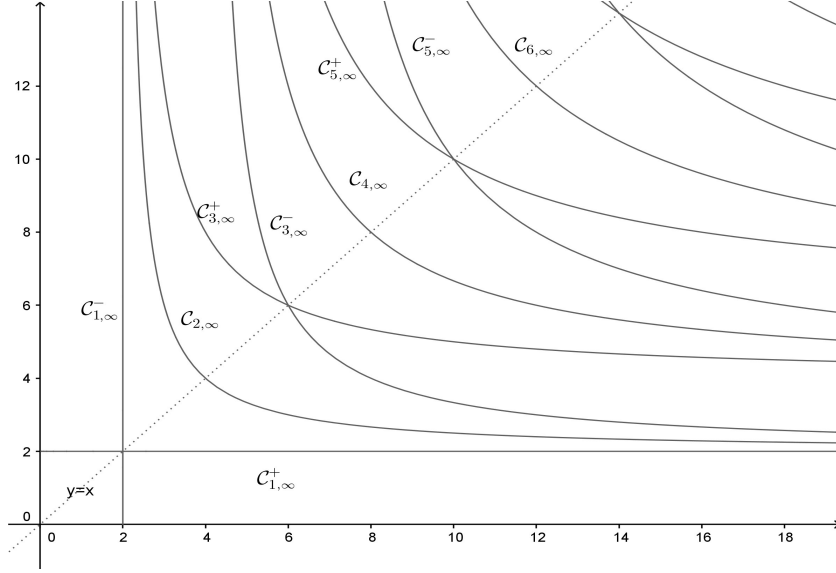
FIGURE 3. \Sigma_\infty for the unit interval in \mathbb{R} .
