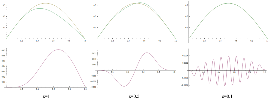
FIGURE 3. The first eigenfunctions and the difference between them for different values of \varepsilon .
