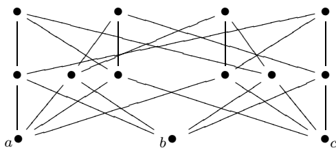
Figure 7.2: A finite model of \mathbb{R}P^2 .
