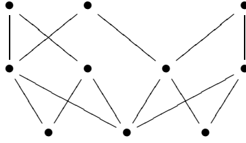
Figure 4.4: W \setminus \{x\} .
