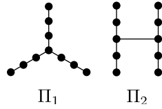
Figure 4.3: Minimally not probe interval trees.
