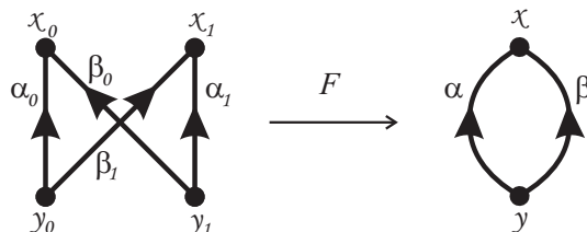
FIGURE 1. A covering from a poset to a category which is not a preorder.
