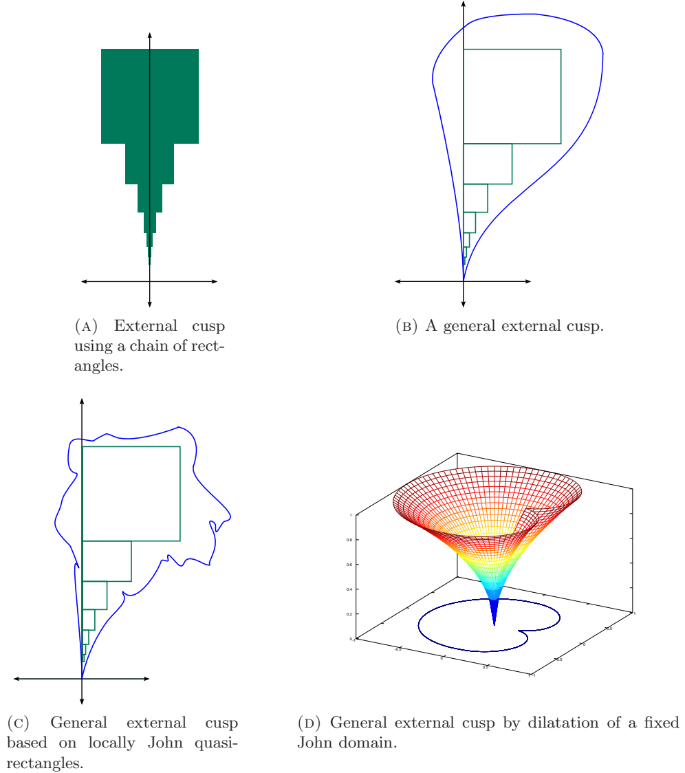
FIGURE 4. Examples of General External Cusps
