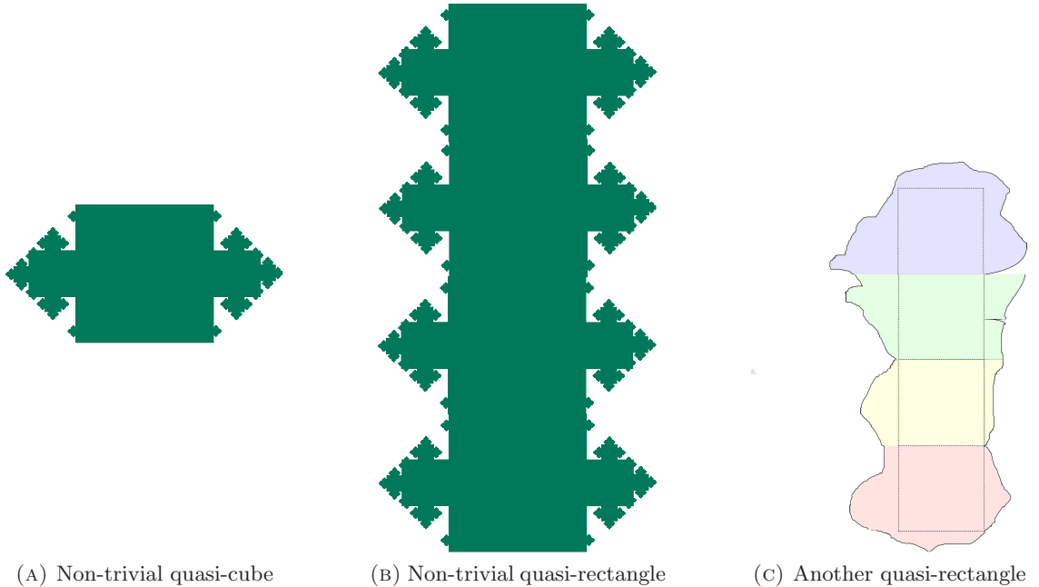
FIGURE 2. Quasi-rectangles
